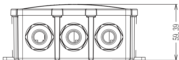
SECTION B-B
